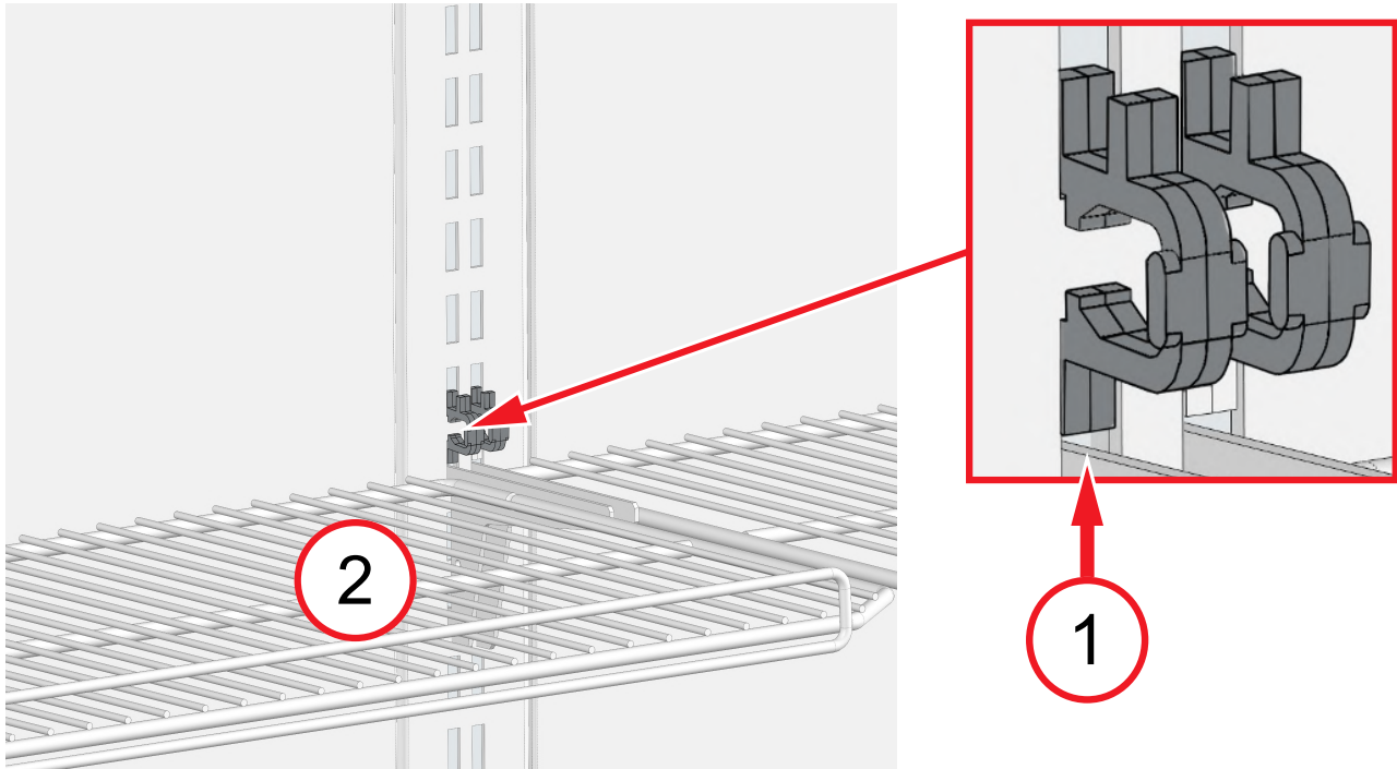
Fig. 1: Transport lock (1) for shelf display (2)
